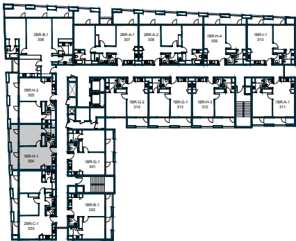
3RD FLOOR LEVEL
