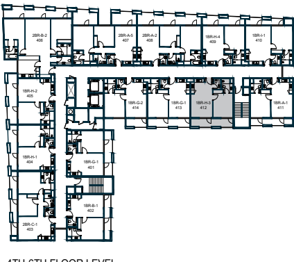
4TH-6TH FLOOR LEVEL
