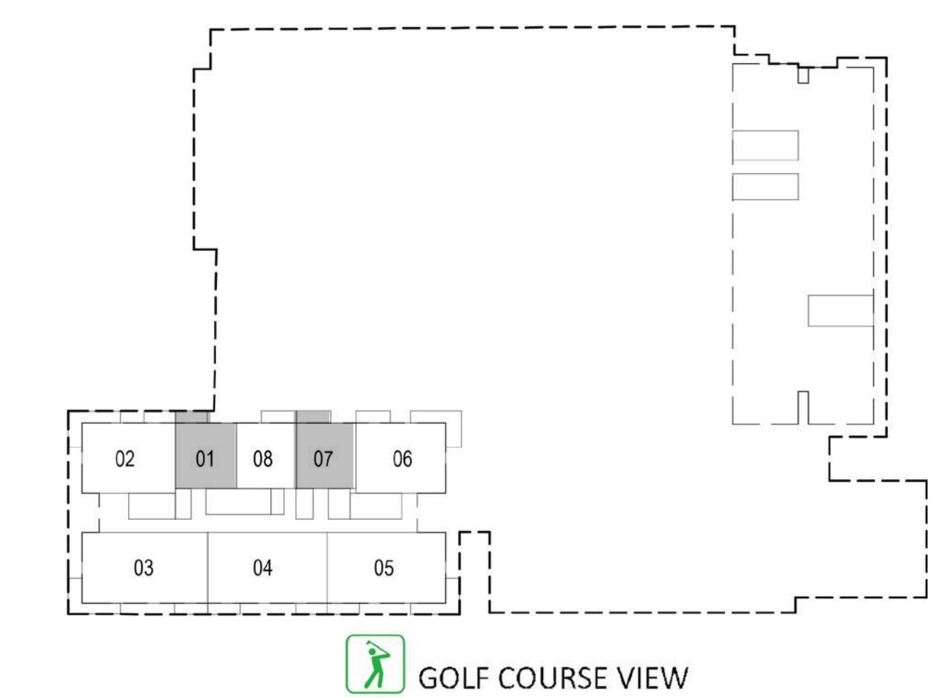
LEVELS 12-14
